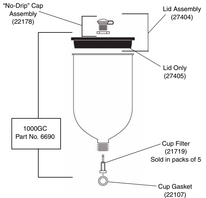
Model 1000GC (6690) (Optional Accessory) Aluminum Gravity Cup (33.8 oz., 1 L)
