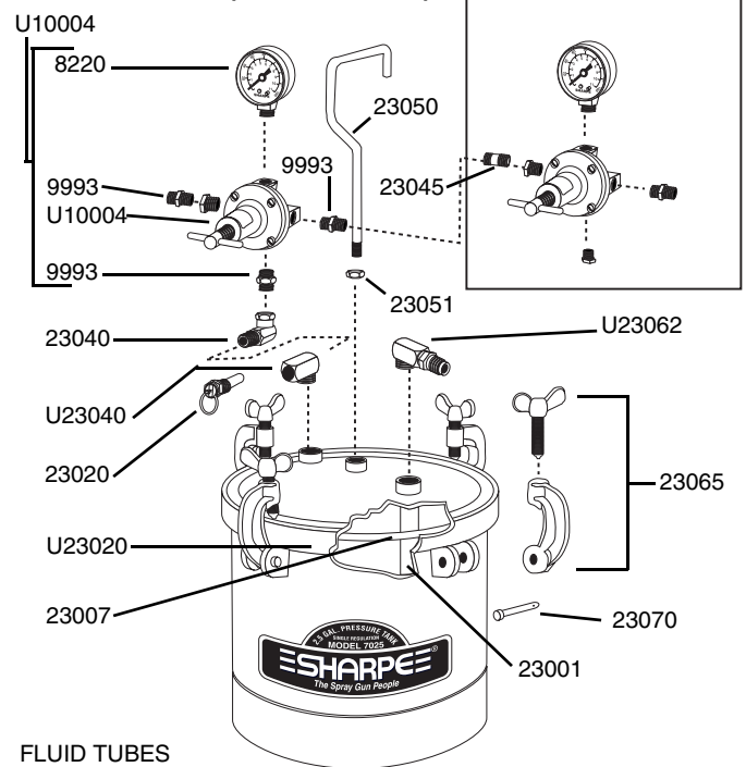
MODEL 7025 & 7027 2.5 & 5.0 GALLON PRESSURE TANK (NON A.S.M.E.) SINGLE & DUAL REGULATION
